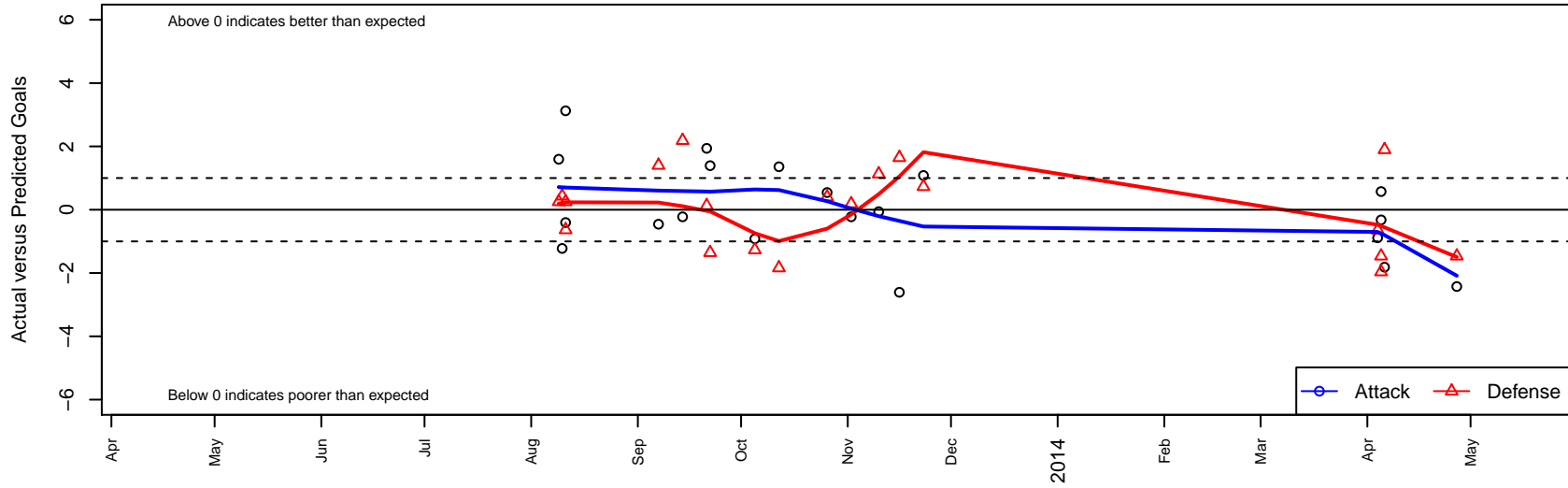
Pumas 03 UNAM B02 Dots are actual minus expected GF (blue circles) and GA (red triangles). Blue line is smoothed change in attack strength. Red is smoothed change in defense strength.
